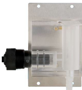
Figure 2: Constant-head flow cell
