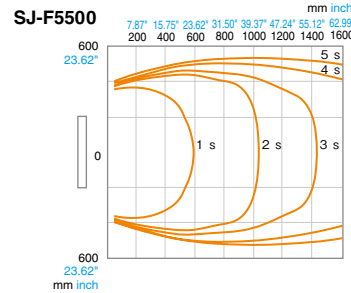
High Speed / High Accuracy Wide Static Elimination Blower SJ-F5500 Series
