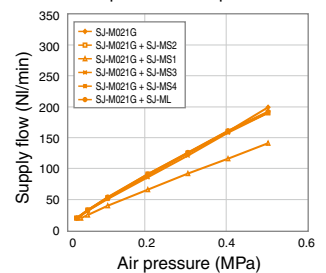
Relationship between air pressure and flow
