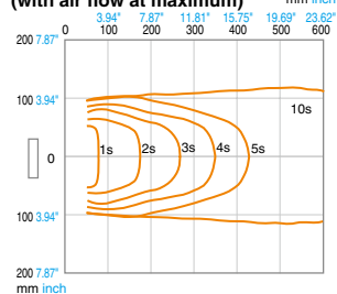
Static elimination area and time (with air flow at maximum)
