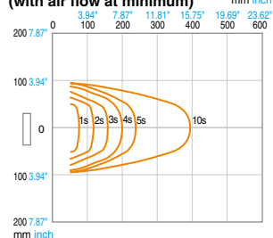
Static elimination area and time (with air flow at minimum)
