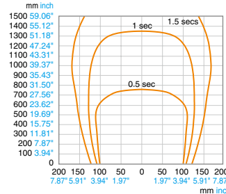
Static elimination area and time (50 Hz)
