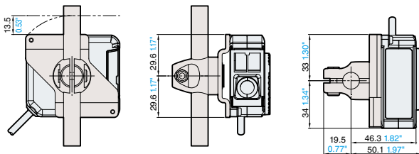
Adjustable Bracket (Mounted) OP-88319
