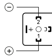
right-angle plug
