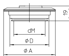
VARIVENT® connection for VARILINE® case
