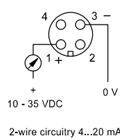
with transmitter
