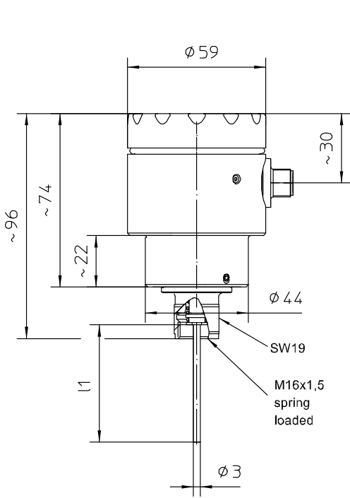
process connection back
