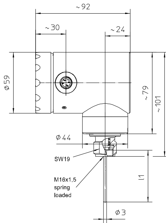
process connection bottom
